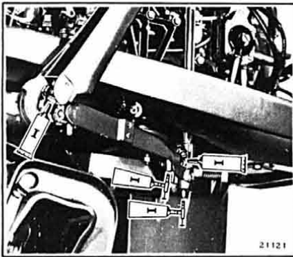
Figure 2-5. Throttle Shaft Bushings and Gears
