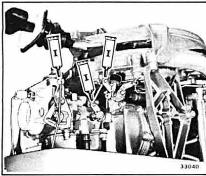
Figure 2-3. Cam Follower, Choke and Linkages
