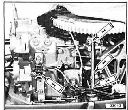
Figure 2-10. Gear Shift Lever Lockout
